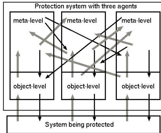
Figure 4: Catriona Kennedy's PhD showed how a software protection system could use "mutual meta-management" to improve resistance to attack. Upward pointing grey arrows represent monitoring, and downward pointing black arrows represent acting. Not all possible arrows are shown.
