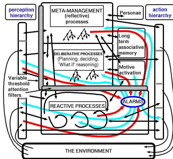
Figure 3: A sketchy representation of a human-like architecture specification, H-CogAff, developed within the CogAff project. Alarm mechanisms can produce different types of episodic emotions. The architecture grows itself.
