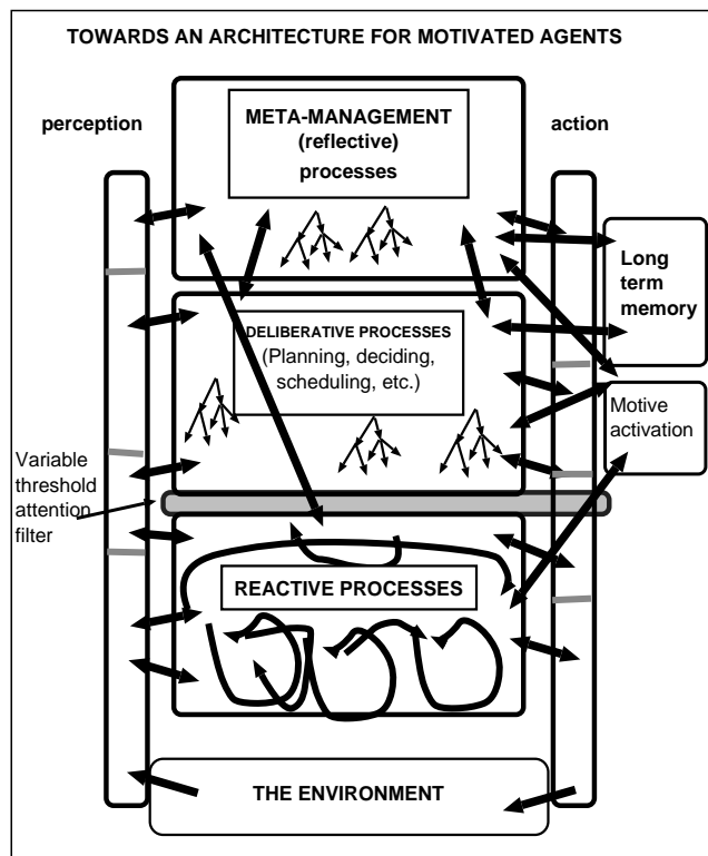
Figure 4: Adding a meta-management layer for self monitoring, self-evaluation, etc. (Alarms not shown, to save clutter.)
